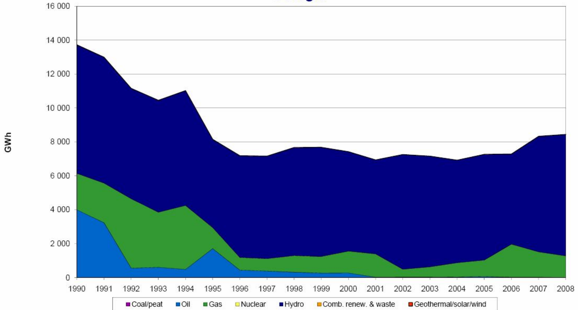
Electricity generation by fuel Georgia
