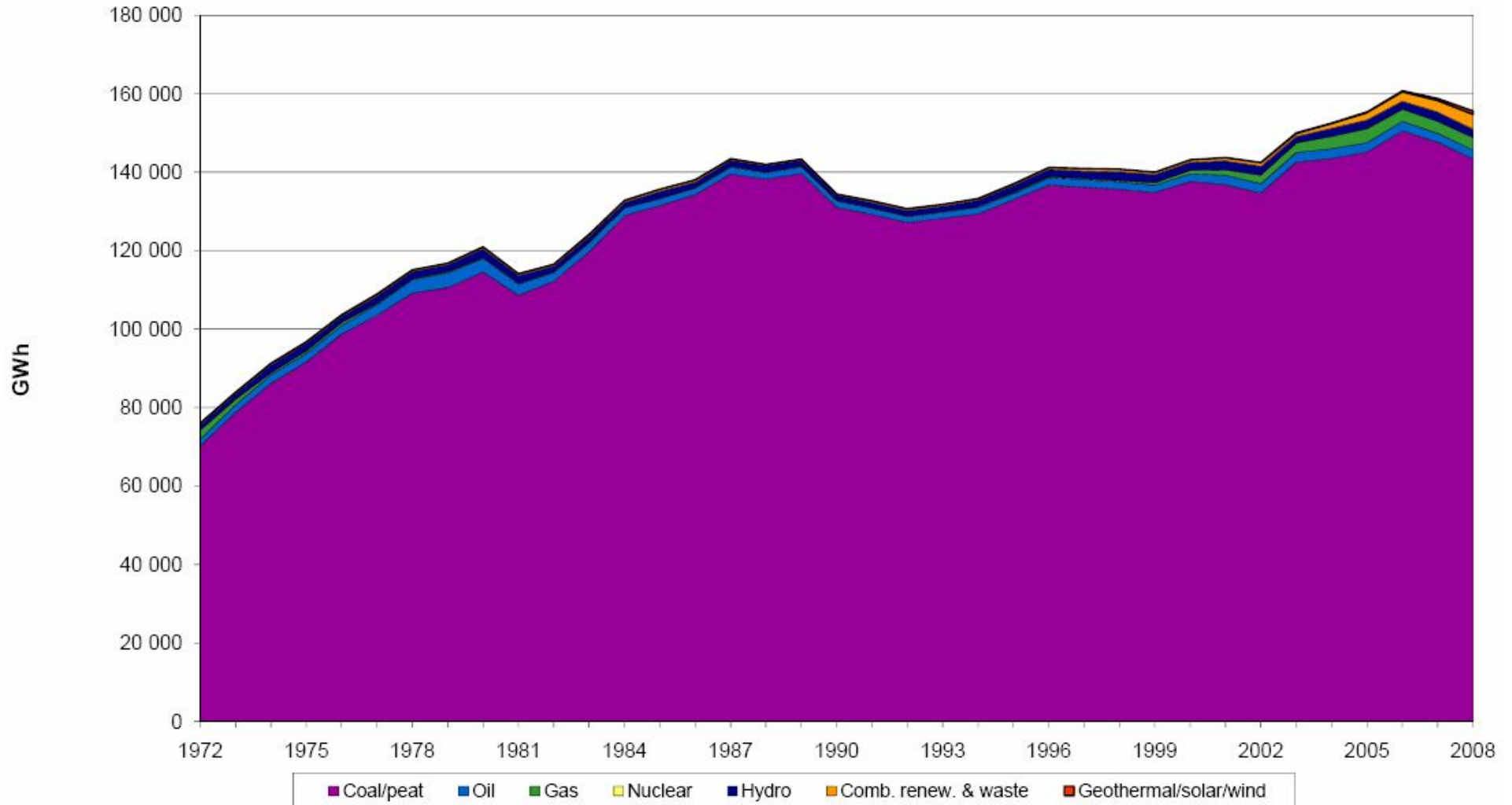
Electricity generation by fuel Poland
